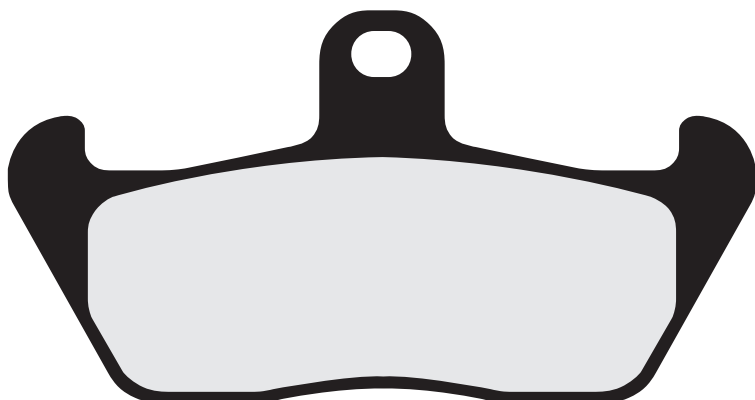
FRDB2640 • 99.50 x 52 x 7.80mm
