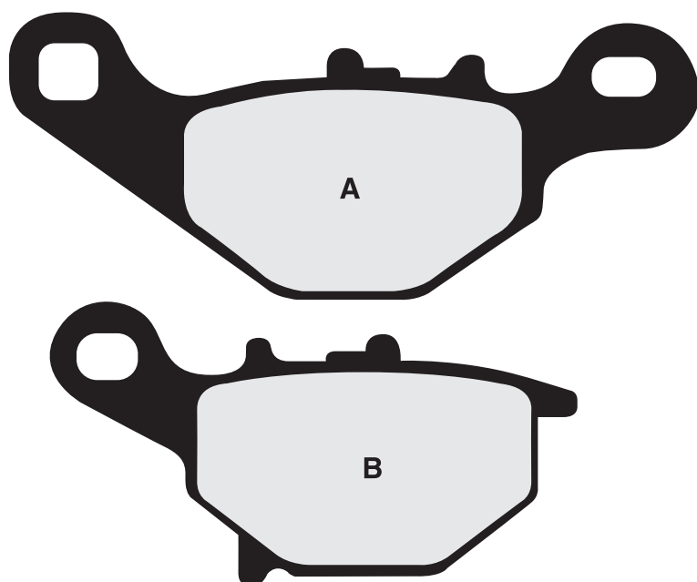
FRDB2250 • A. 99.00 x 44.10 x 7.56mm B. 75.50 x 37.90 x 8.26mm
