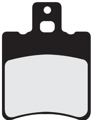
FRDB2610 • 39.80 x 53.70 x 6.40mm
