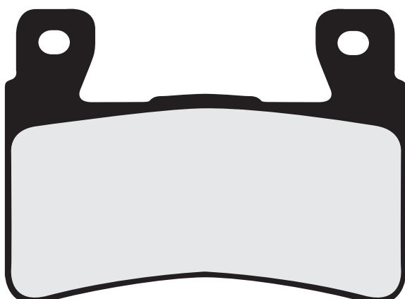
FRDB2048 • 74.75 x 55.40 x 7.60mm
