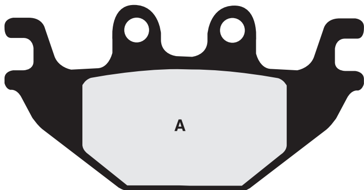
FRDB2530 • A. 94 x 46 x 8.50mm - B. 73 x 46 x 11mm
