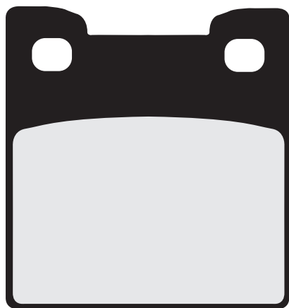
FRDB2081 • 52.60 x 56.30 x 9mm
