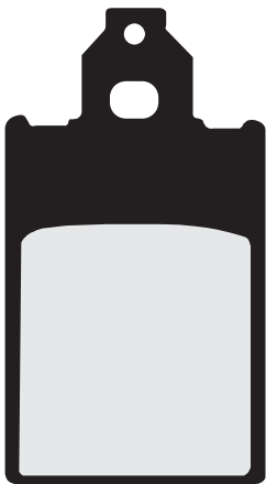
FRDB2660 • 31.50 x 57.20 x 5.50mm
