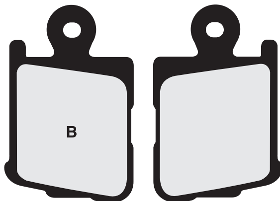
FRDB2203 • A. 69.20 x 51.55 x 8.90 - B. 33 x 51.55 x 8.90mm
