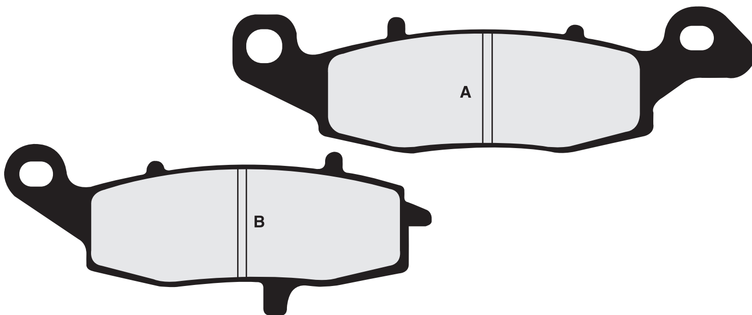
FRDB2730 • A. 133.50 x 36.80 x 8.40mm - B. 109.60 x 51.75 x 8.50mm
