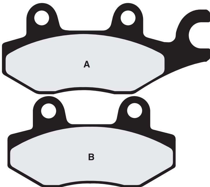
FRDB2480 • 77.30 x 42.20 x 7.20mm
