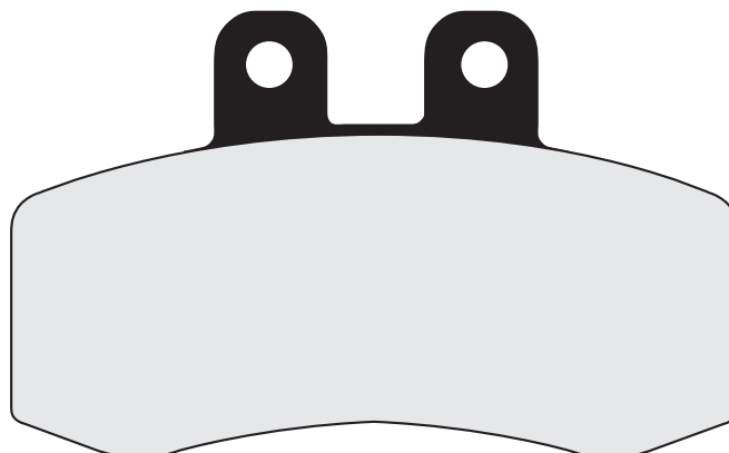
FRDB2085 • 87 x 53 x 7.50mm
