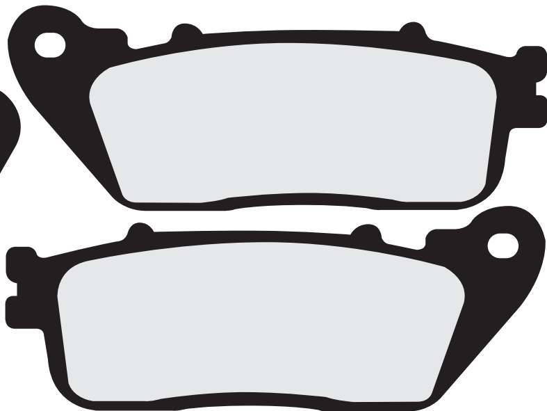
FRDB2192 • 99.35 x 38.65 x 8.90mm
