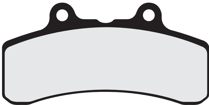
FRDB2178 • 112.10 x 56.30 x 10mm
