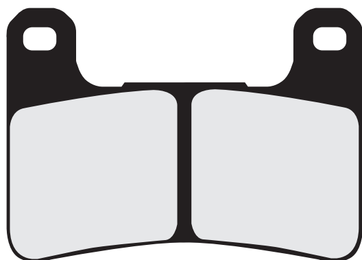
FRDB2118 • 71.45 x 49.90 x 7.76mm
