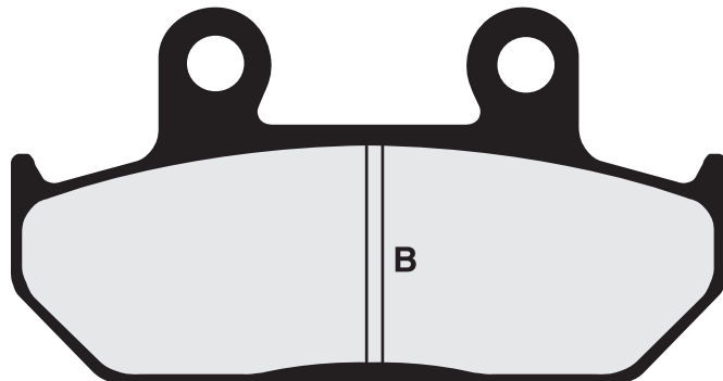
FRDB2690 • A. 104 x 45.60 x 9.80mm - B. 88 x 42 x 9.80mm
