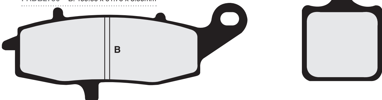
FRDB2750 • B. 109.60 x 51.75 x 8.50mm
