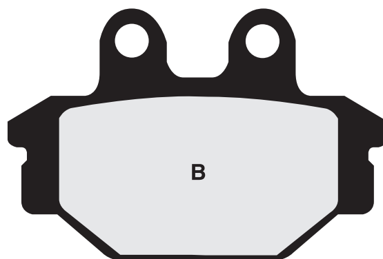
FRDB2530 • A. 94 x 46 x 8.50mm - B. 73 x 46 x 11mm
