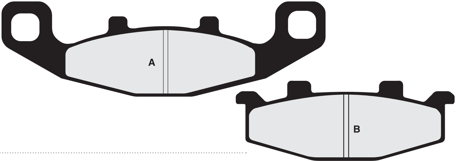
FRDB2740 • A. 118 x 48 x 8.60mm - B. 97.50 x 57 x 10.80mm
